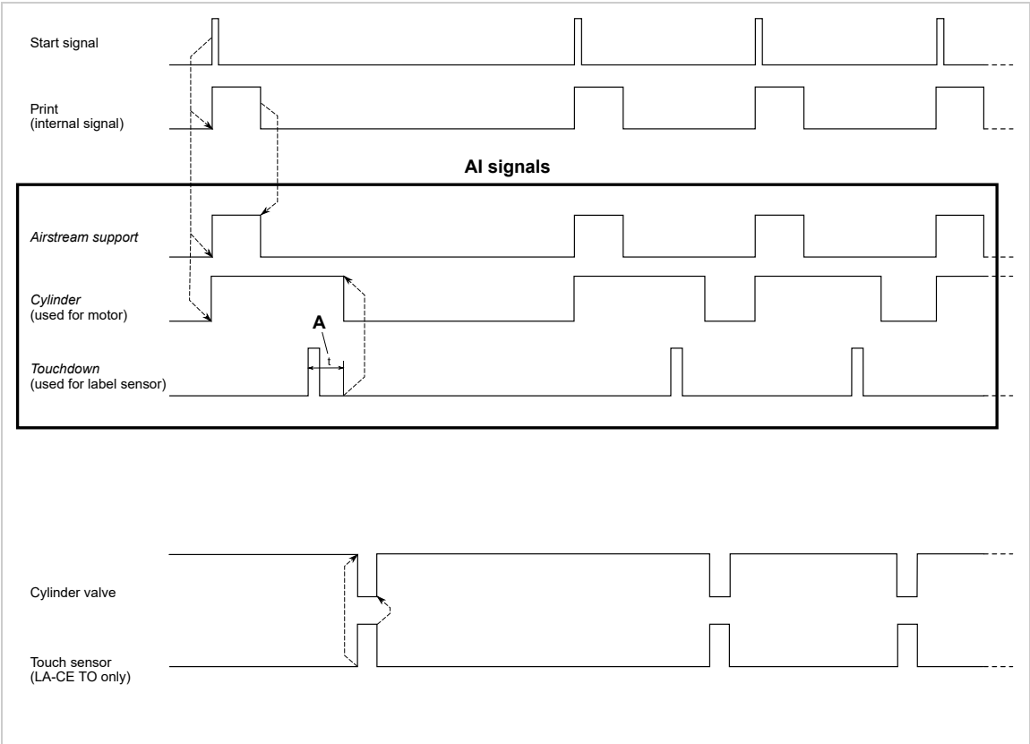
[33] Pattern of control signals over time LA-CE or LA-CE TO applicators.
