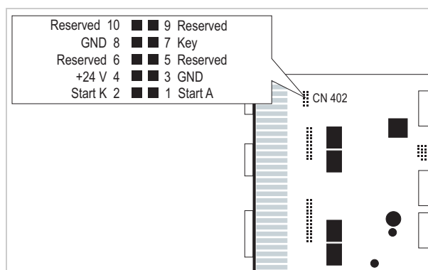
[22] Position and pin assignment of the internal product sensor connection (CN 402).
