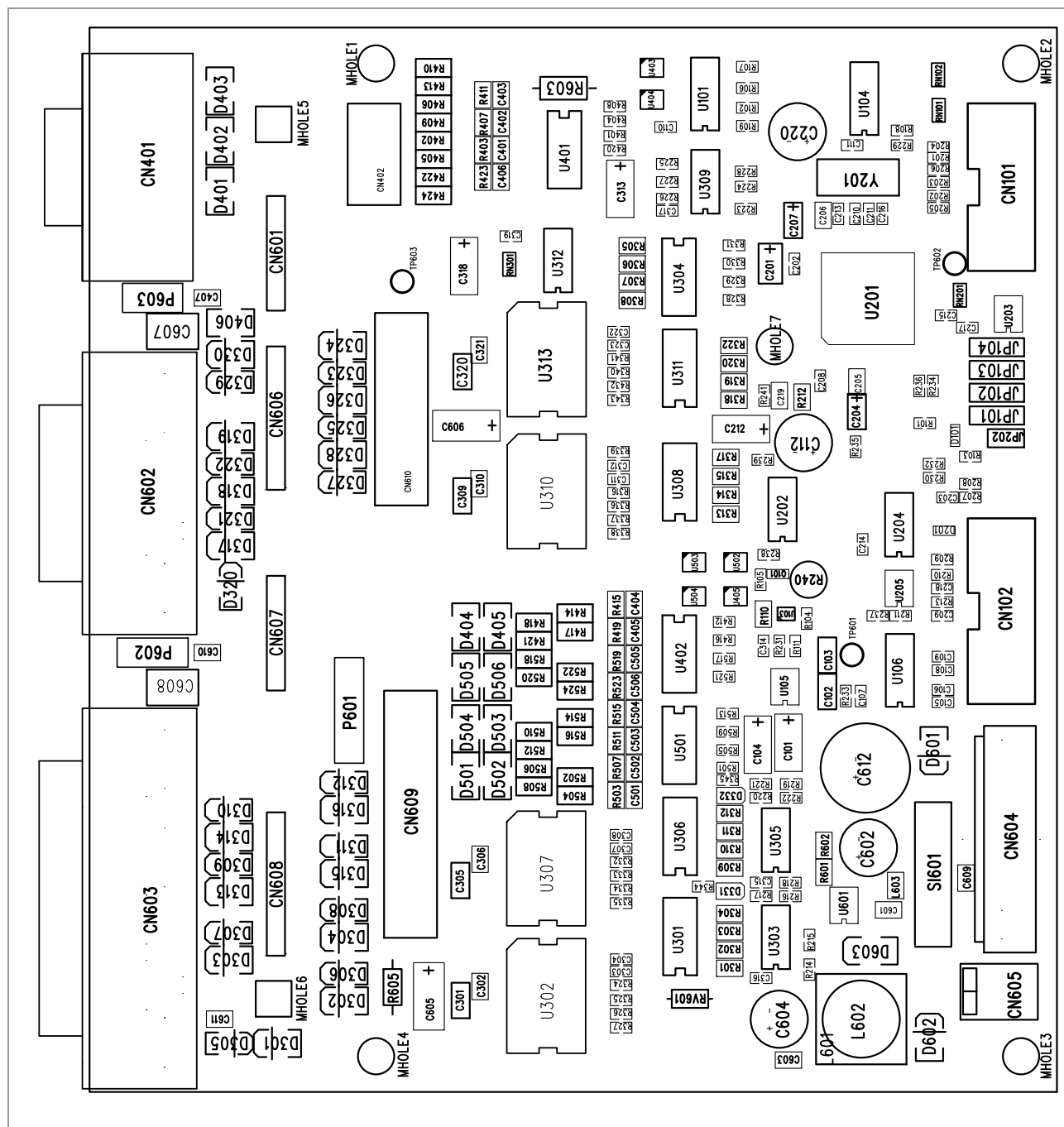
[7] Layout diagram for Applicator Interface (PCB = A3417-03)
