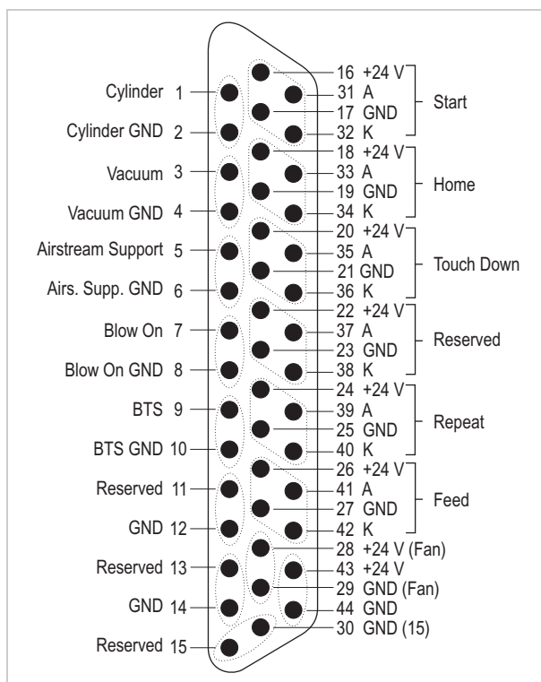
[13] Pin assignment applicator connection.
