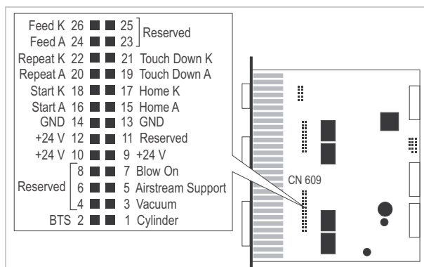
[14] Position and pin assignment of the internal applicator connection (CN 609).
