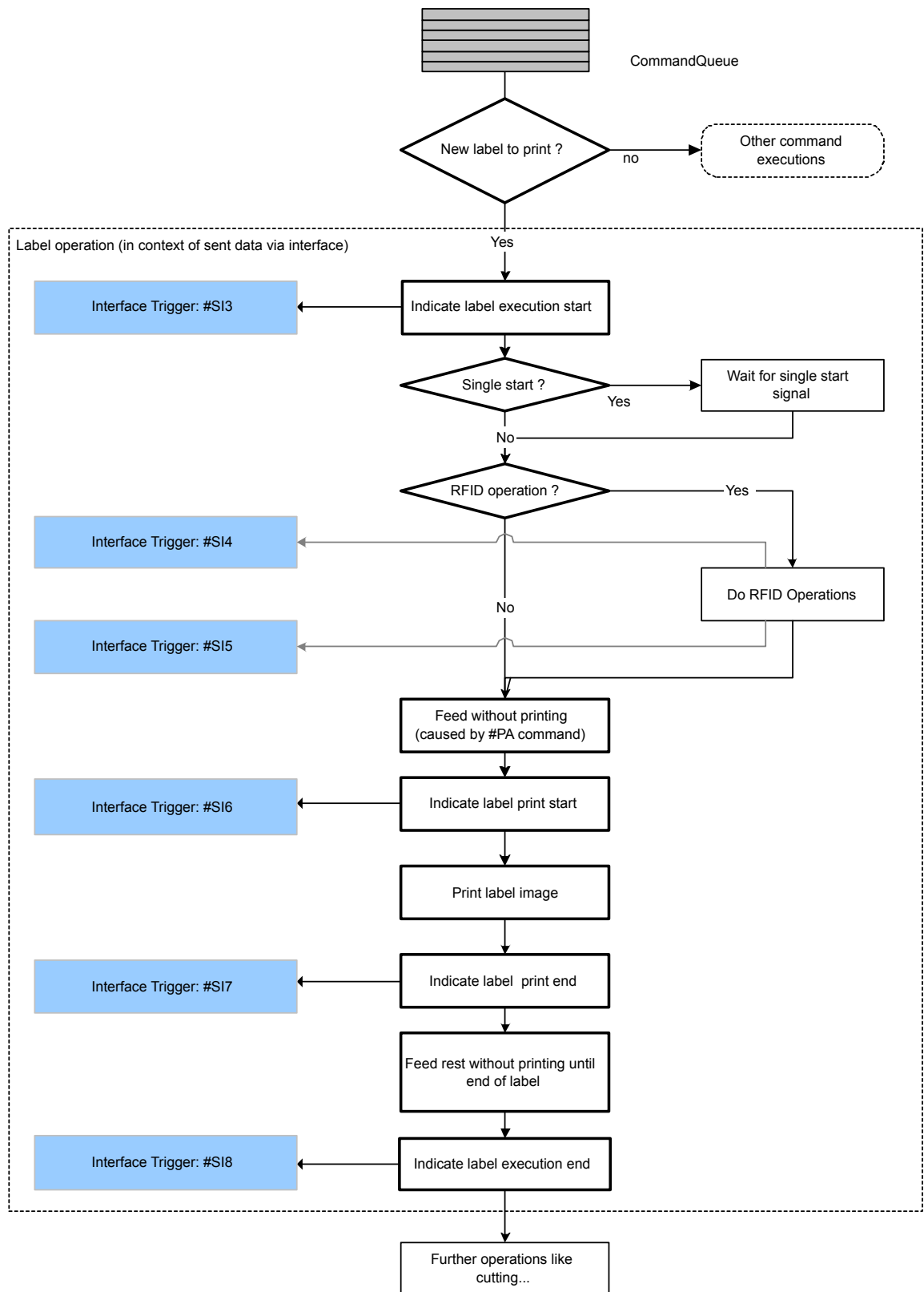
Fig. 10: Flowchart showing label operation trigger points #3 - #8.
