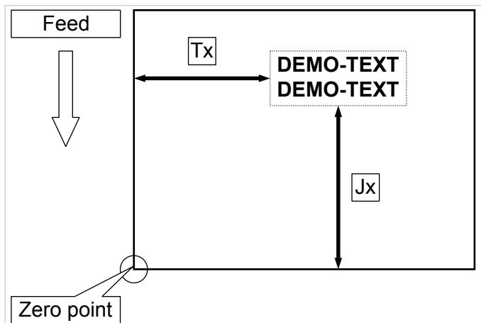
Fig. 6: Vertical (Jx) and horizontal (Tx) print position on the label.
