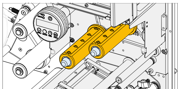
[21] Folienkern-Adapter.
